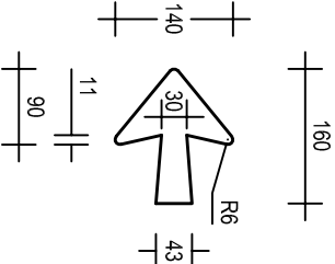
Arrow Detail
